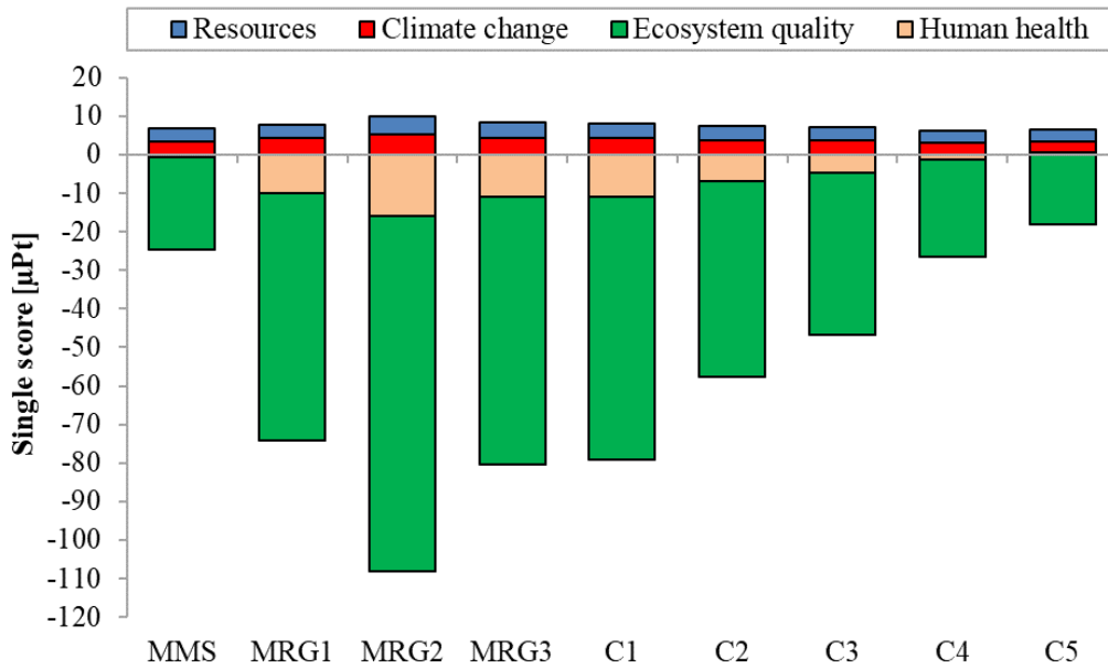
Figure 4: The single score results of the life cycle impact assessment
