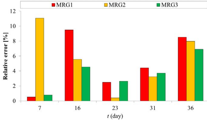
Figure 3: The relative error values between measured and modelled methane content data in the gas phase
