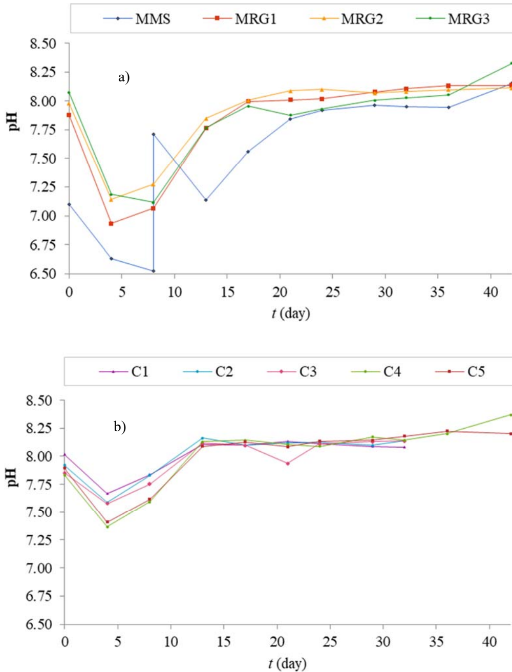
Figure 2: Profiles of pH values in digested substrates during a) mono- and b) co-digestion
