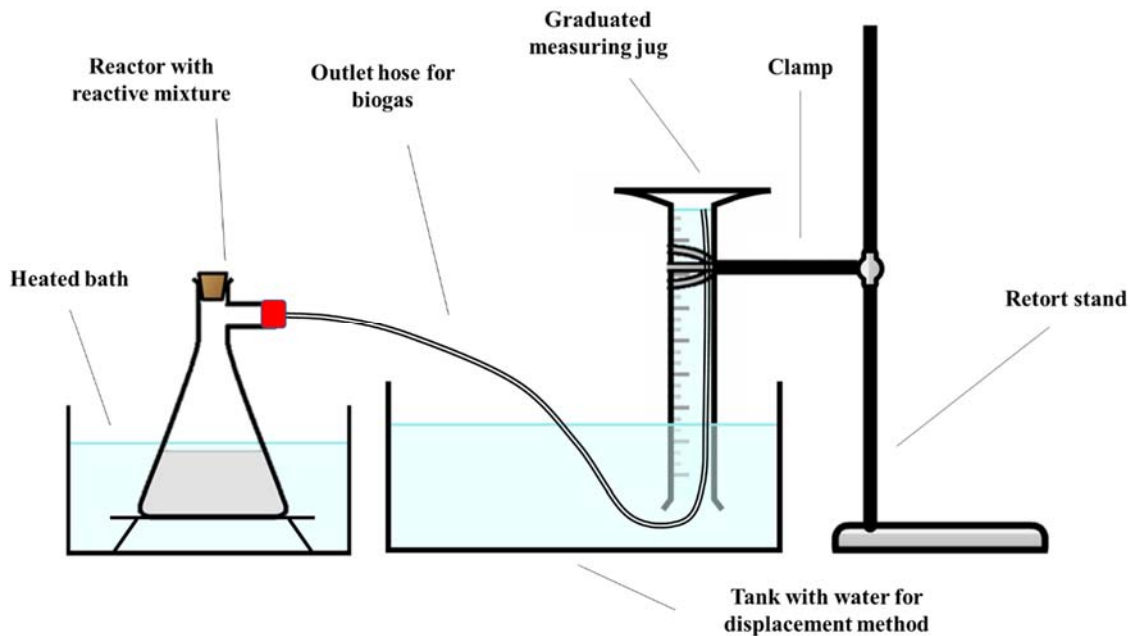
Figure 1: Laboratory experimental set-up for anaerobic digestion
